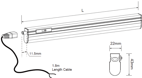
Dimension Diagram
